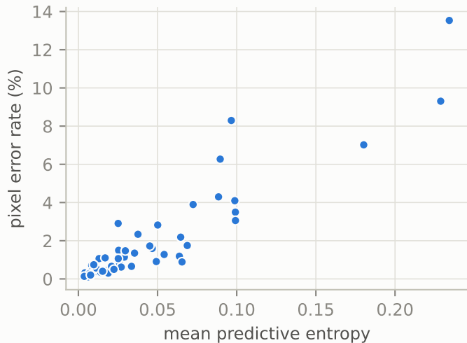
Per-image: entropy vs error ( r = 0.93 )
